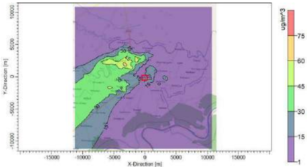
Fig. 11: Predicted PM Concentrations from All Brick Kilns (103) with Dominant Wind in North-East Sector in the Study Area
