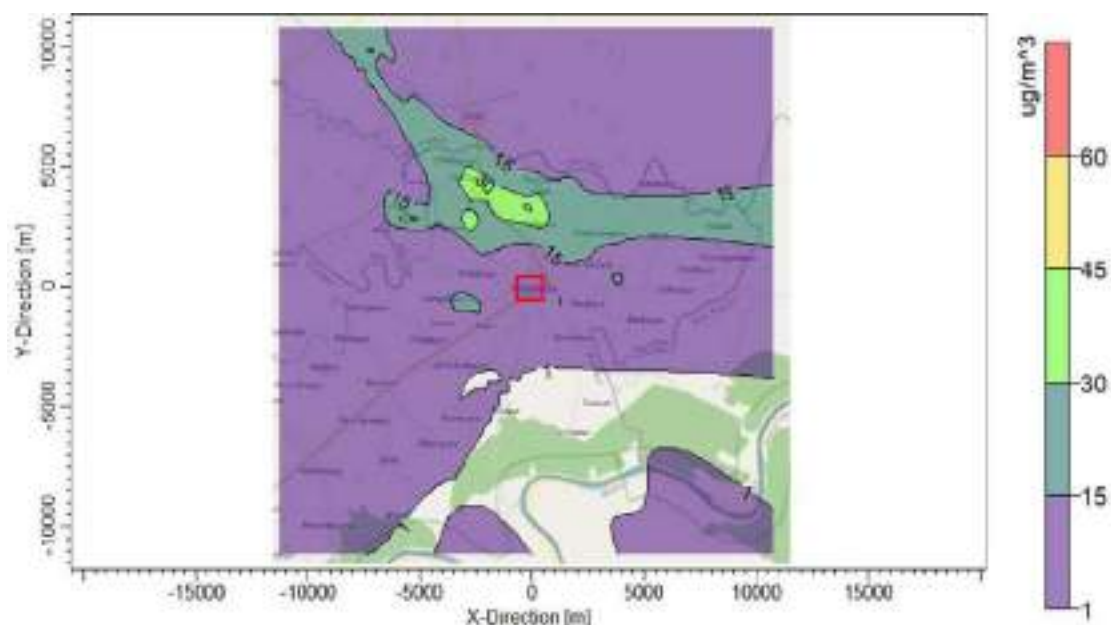
Fig. 12: Predicted PM Concentrations from All Brick Kilns (103) with Wind equally distributed in All Directions in the Study Area
