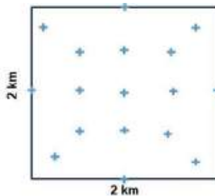
Fig. 4: Discrete Receptor Points for Rajakhhera Village (8 directions with 500 m interval + Centre)
